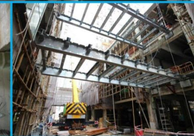
Five Link Bridges Connecting Mills 5 & 6
